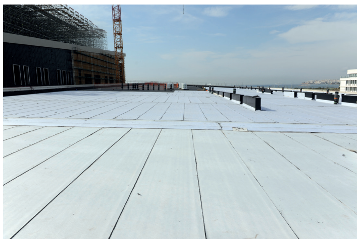
Application of bituminous membrane ESHADIEN SP GEO at SNFCC Niarchos
